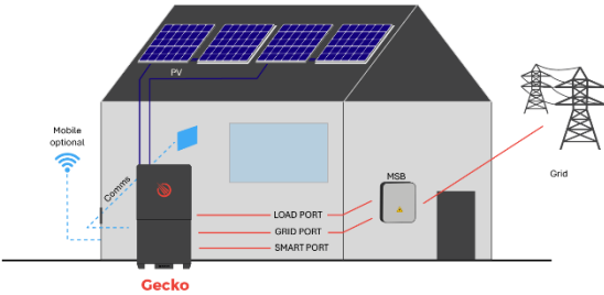
On-grid example
