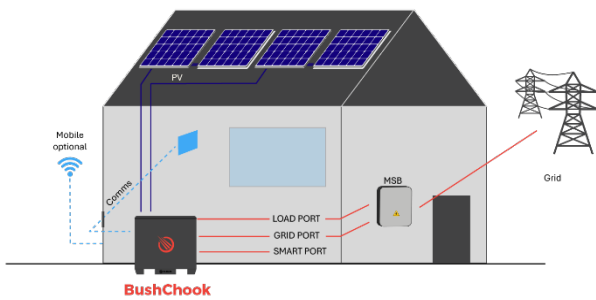
On-grid example
