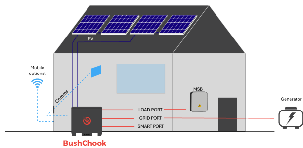
Off-grid example
